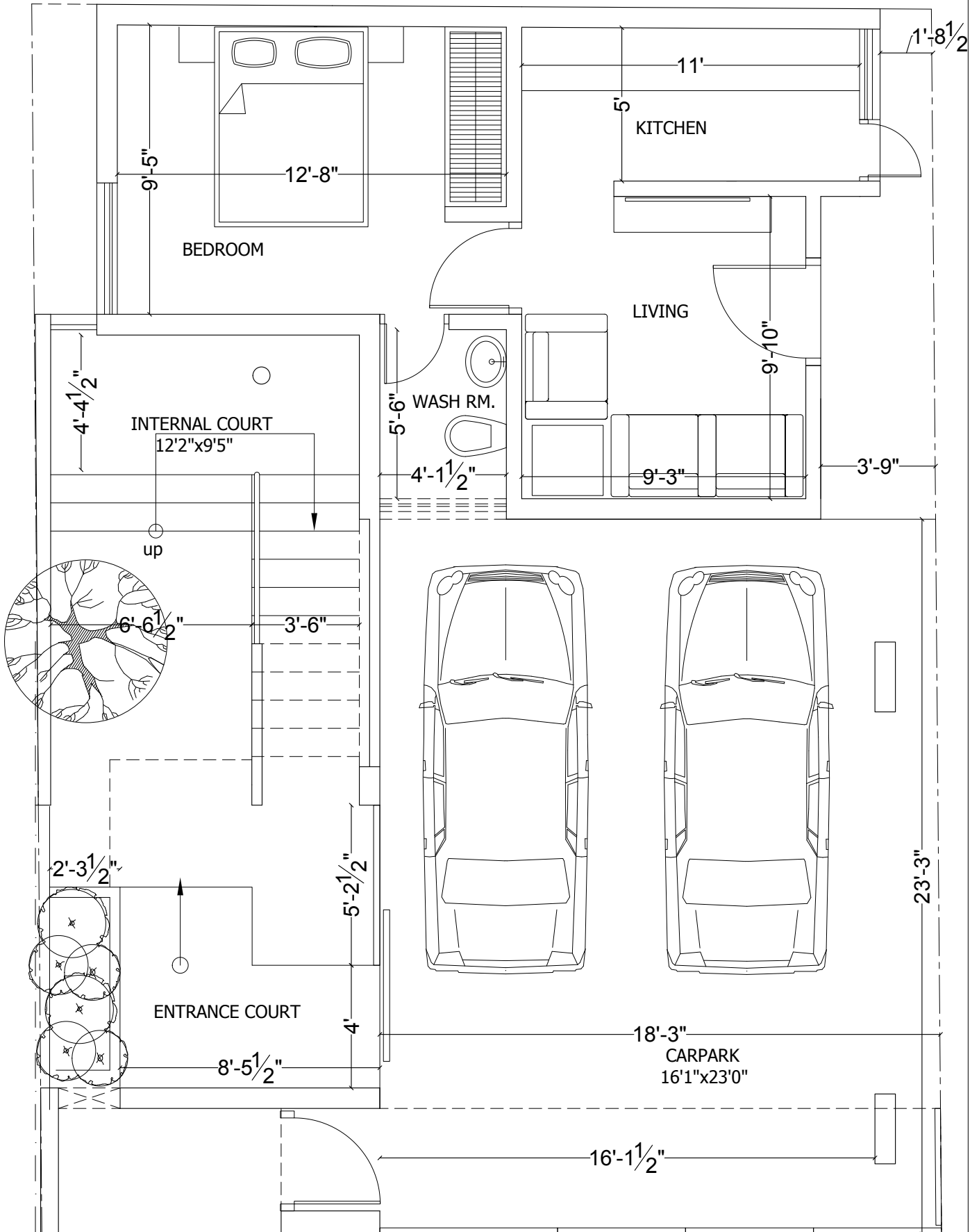
GROUND FLOOR PLAN (option 2) Mrs. & Mr. Sooraj
