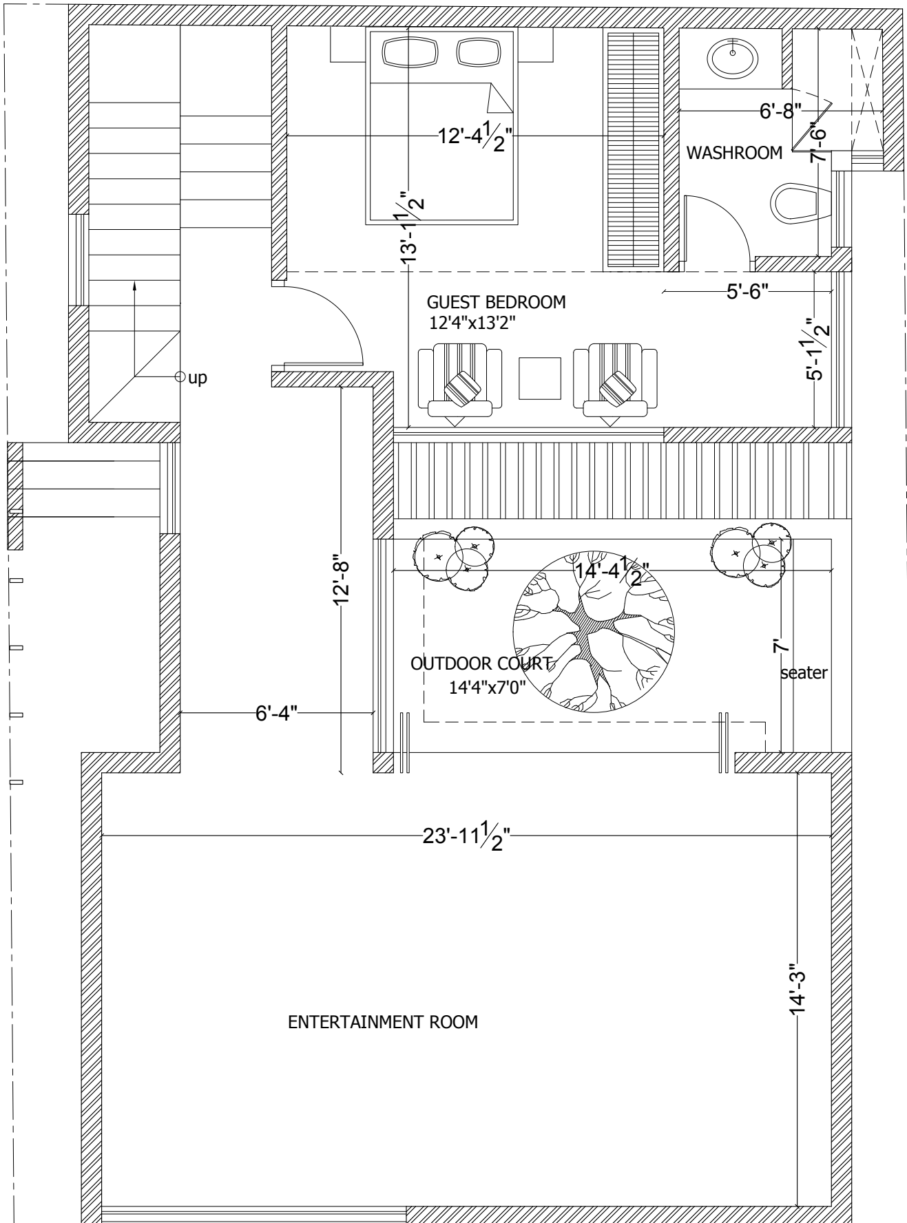
THIRD FLOOR PLAN Mrs. & Mr. Sooraj
