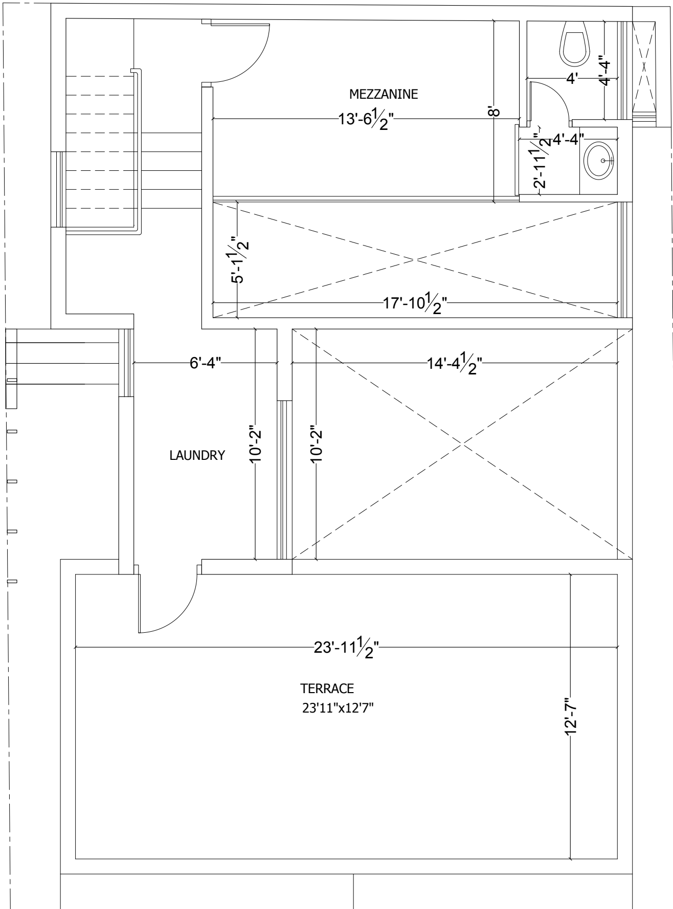
MEZZANINE AND TERRACE FLOOR PLAN Mrs. & Mr. Sooraj
